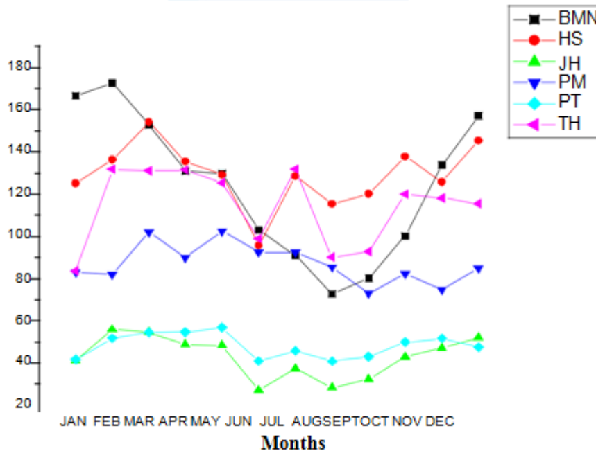
Fig. 1: Graph of mean monthly annual reference evapotranspiration estimated by different methods for Umuahia station.
